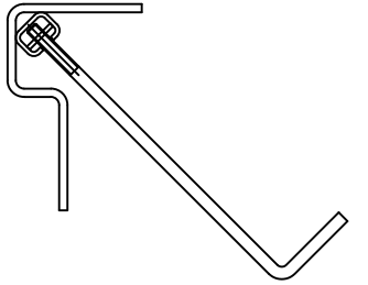
Brick-in Option Detail X
