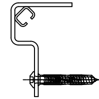
Build-in Option Detail X
