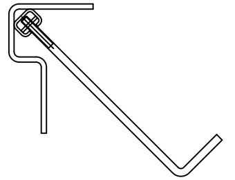
Brick-in Option Detail X
